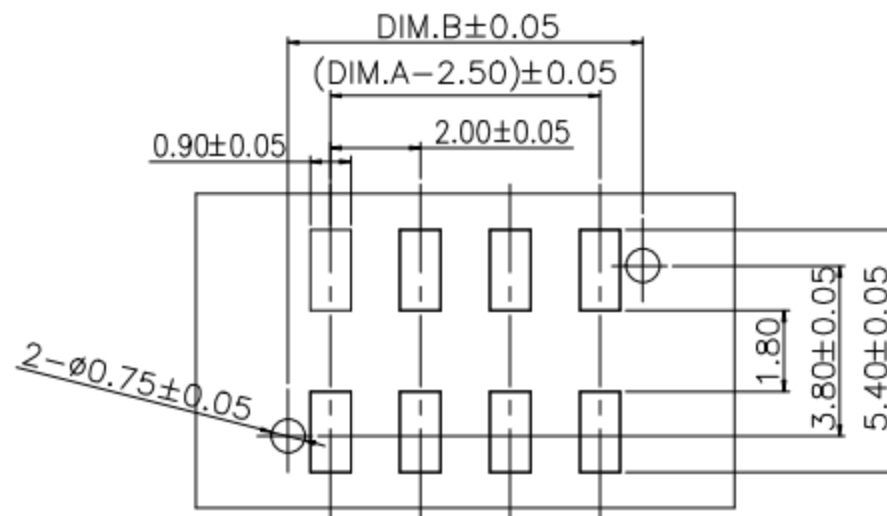
P. C. B LAYOUT TOLERANCE: \pm 0.05
